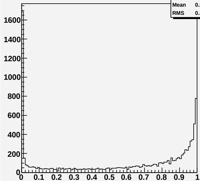
probchi2d
