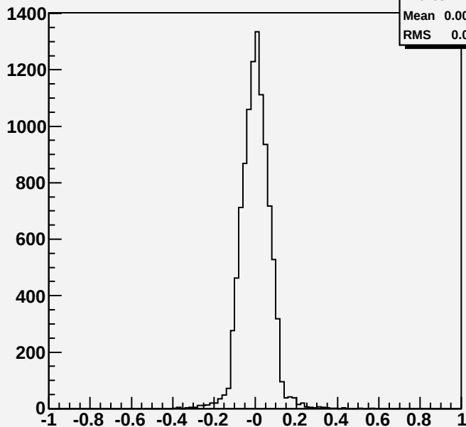
slopediff
