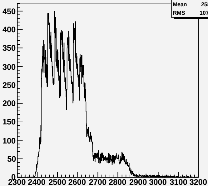
timeboxtest
