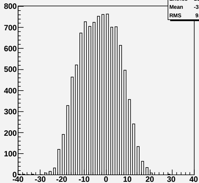
m_chi2_bphi
