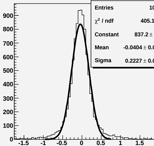
residuinew
