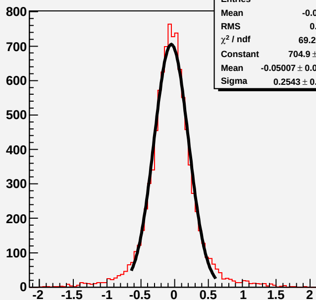
residuietest
