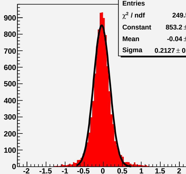
residuinew
