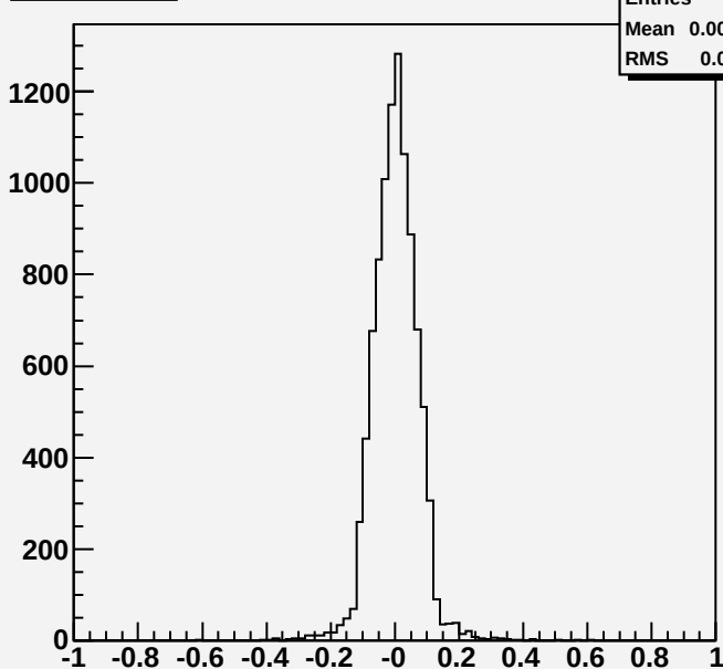
slopediff
