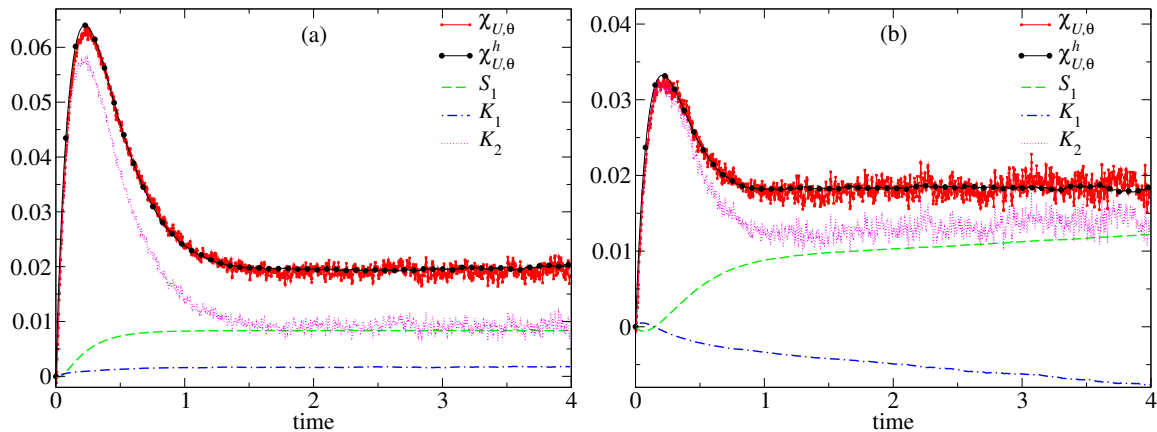
Figure 1. Temperature susceptibility of the energy U(x) = \cos x of a single particle, computed with the formula ( \chi ) and by actually perturbing the system ( \chi^h ). Also the single terms of the formula are shown. The system is out of equilibrium because of a quench at time t = 0 from an initial T_0 = 5 to T = 0.3 . Consistently, the response is not given by twice the correlation S_1 between entropy produced and observable. In (a) there is no additional constant force ( f = 0 ), while f = 0.7 in (b) generates a nonequilibrium steady state previous to the quench. Averages are over 4 \times 10^7 trajectories, integrated with finite time step dt = 2.5 \times 10^{-3} .
