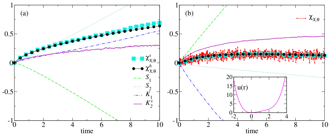
Figure 2. Temperature steady-state susceptibility of the length X of the overdamped chain ( N = 11 ), computed with the formula ( \chi^s ) and by actually perturbing the system ( \chi^h ). Also here the single terms of the formula are displayed. In these examples, T_i varies linearly from T_1 = 1 to T_N = 2 . In (a) the response is to a global temperature rise, while in (b) it is to an increase of the gradient T_N - T_1 preserving the average bath temperature (the inset shows the interaction potential). Averages are over 10^7 trajectories, integrated with finite time step dt = 10^{-3} .
