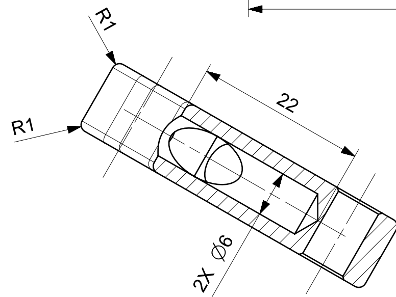
SECTION C-C (SCALE 2:1)
