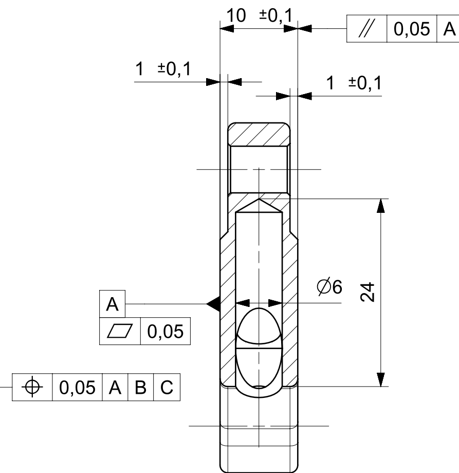
SECTION B-B (SCALE 2:1)
