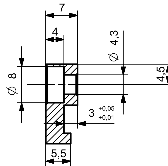
SECTION B-B (SCALE 2:1)
