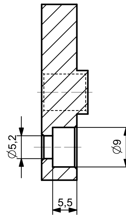
SECTION B-B (SCALE 2:1)
