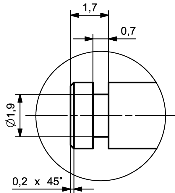
DETAIL A SCALE 10:1
