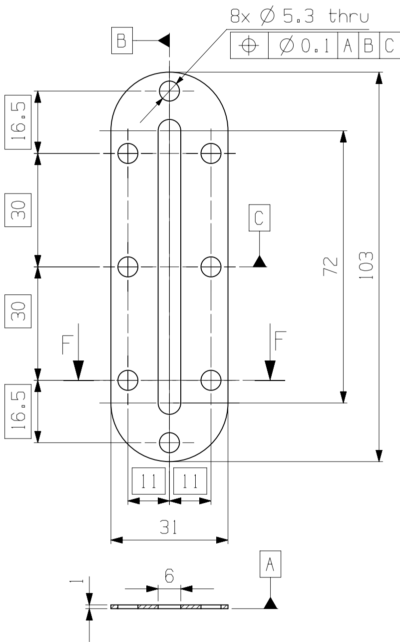
Section F-F
