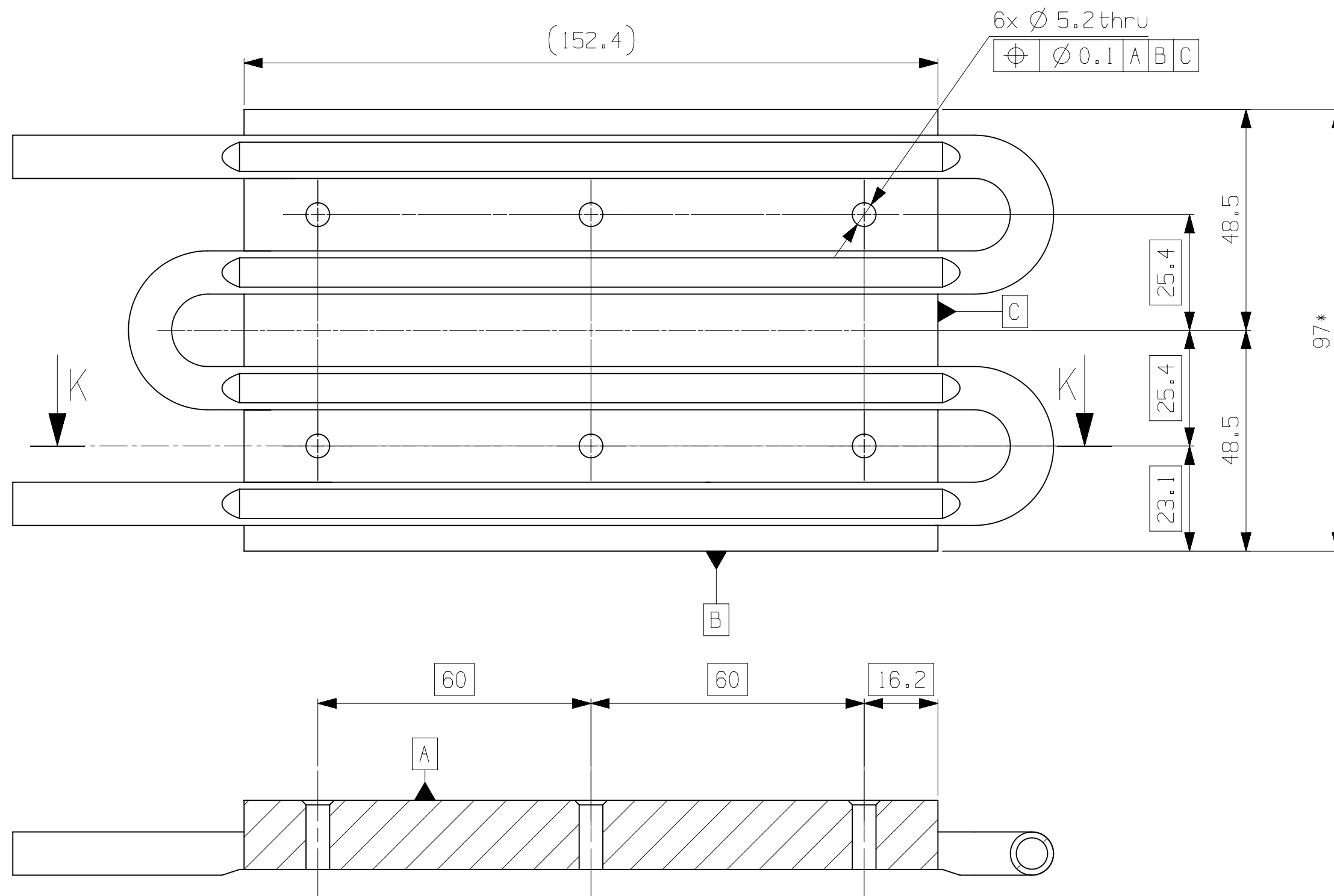
Section K-K
