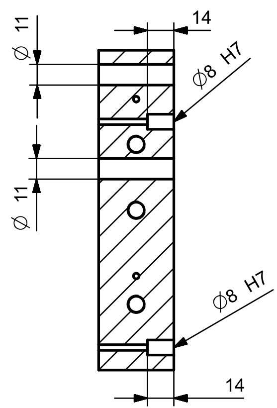
SECTION B-B
