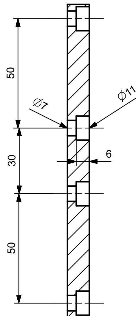
SECTION C-C
