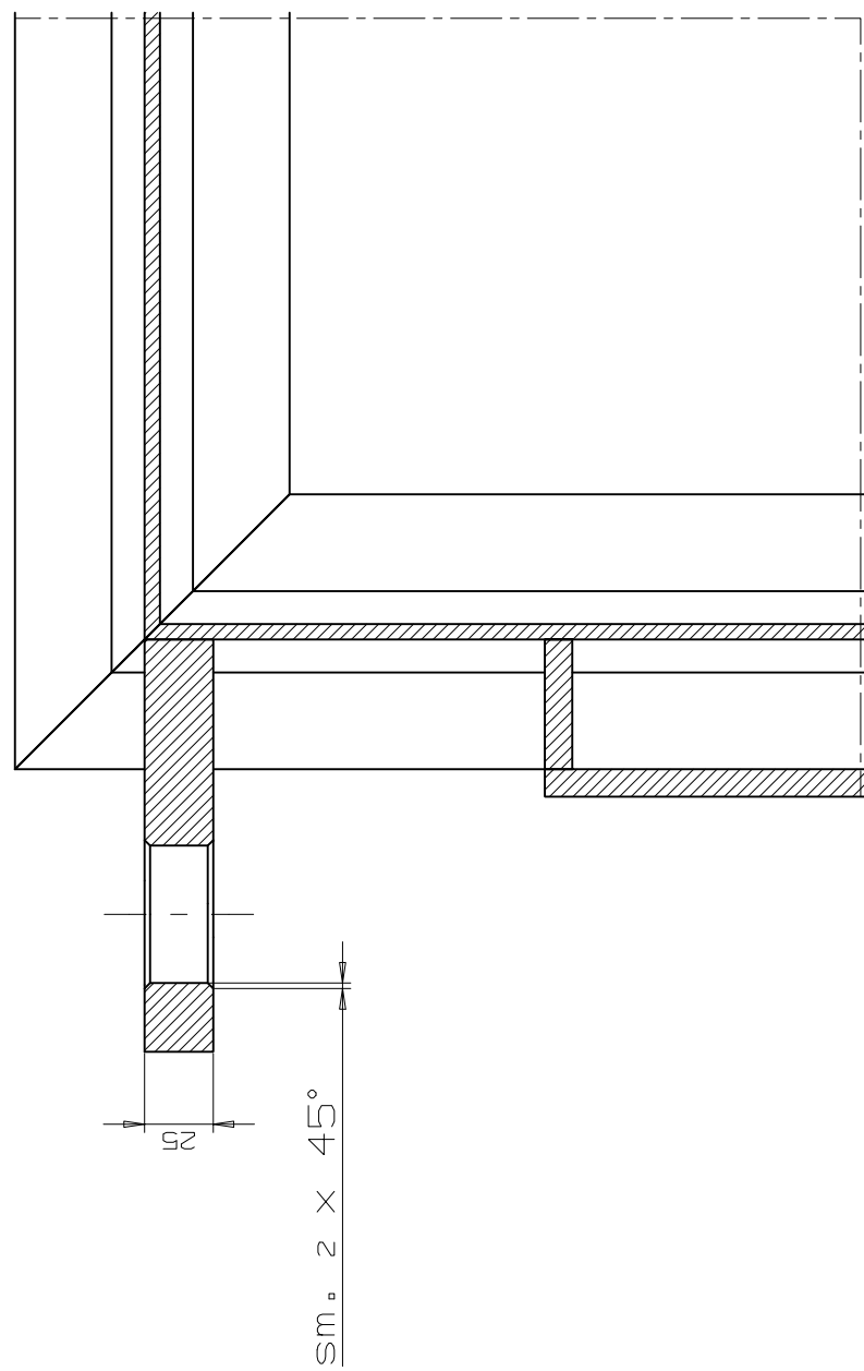
SECTION J-J
