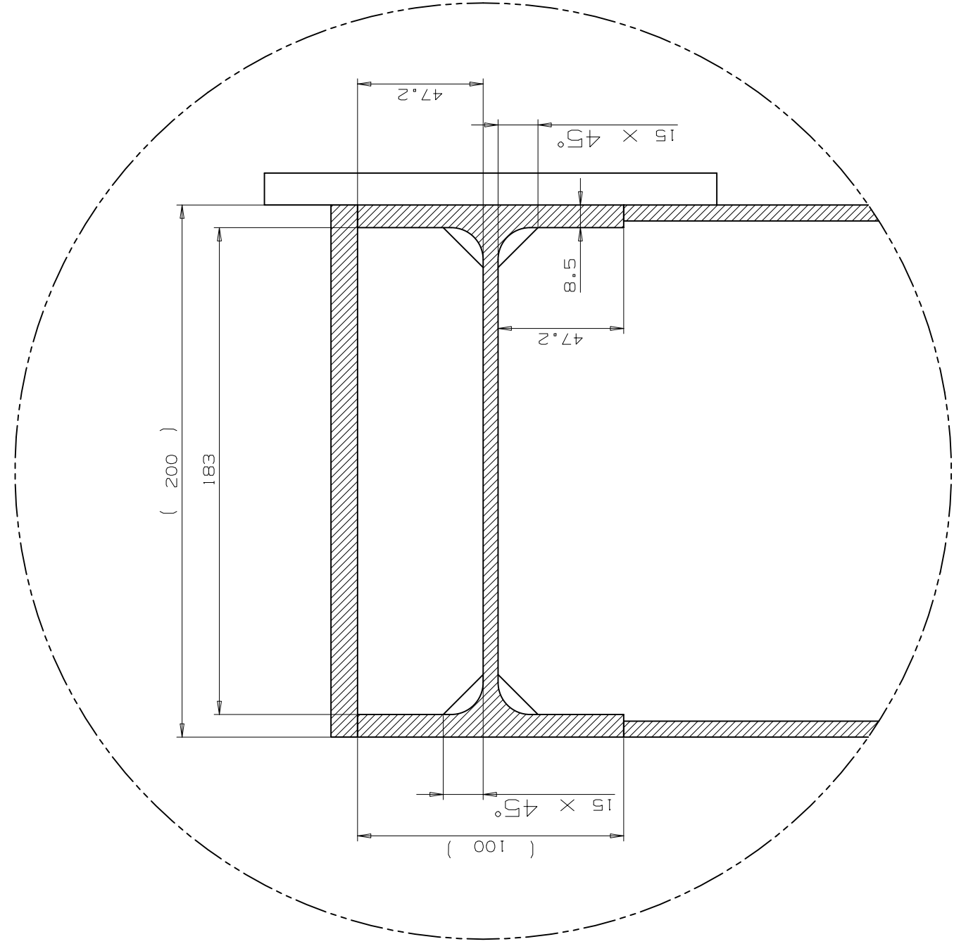
DETAIL G SCALE 1:20
