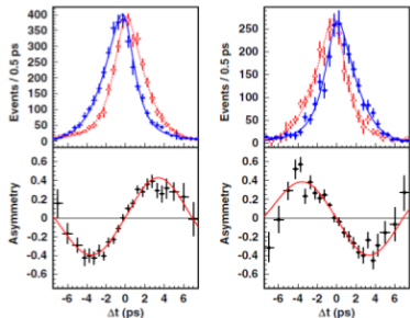
FIG. 2 (color online). The background-subtracted \Delta t distribution (top) for q = +1 (red) and q = -1 (blue) events and asymmetry (bottom) for good tag quality ( r > 0.5 ) events for all CP -odd modes combined (left) and the CP -even mode (right).
