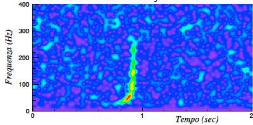
LIGO Hanford
