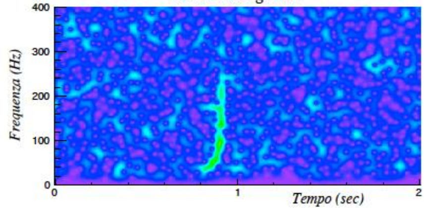
LIGO Livingstone
