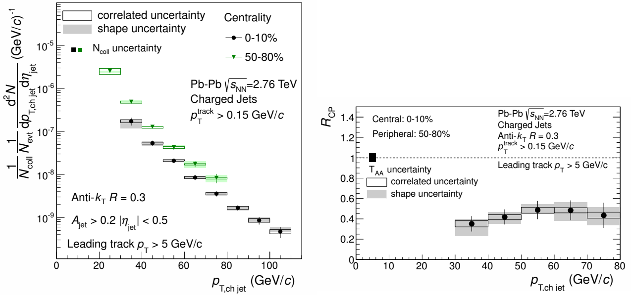
Figure 33. Left panel: transverse momentum distribution of jets reconstructed from charged particles measured by ALICE in Pb+Pb collisions at \sqrt{s_{\text{NN}}} = 2.76 TeV, for central (0-10%) and peripheral collisions (50-80%). The distributions are normalised per nucleon-nucleon collision. Right panel: ratio of the spectra in central and peripheral collisions: nuclear modification factor R_{CP} as a function of transverse momentum.
