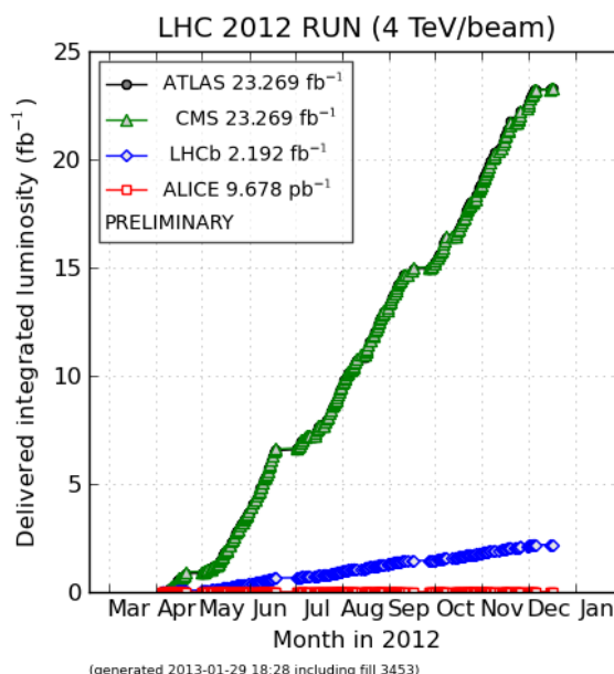
Figure 6. Luminosity during the 2012 run; for ATLAS and CMS the 2011 total luminosity was just 25% of that of 2012.
