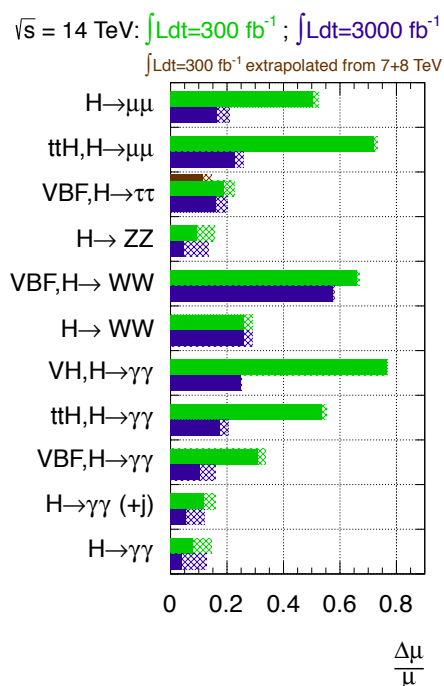
Figure 14. The expected uncertainty, from simulations, on the Higgs signal strength, derived from analyses of 300 fb -1 (green) or 3000 fb -1 (blue) of data, to be collected by ATLAS at 14 TeV.
