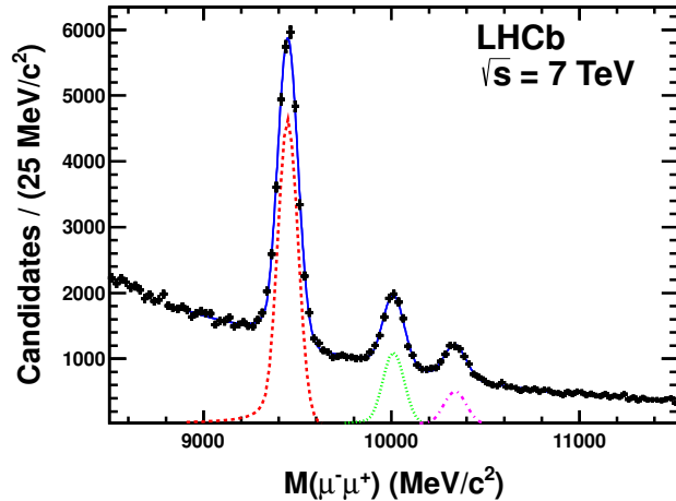
Figure 29. Reconstruction of the di-muon invariant mass illustrating the resolution to observe the Upsilon 1S, 2S and 3S resonances.
