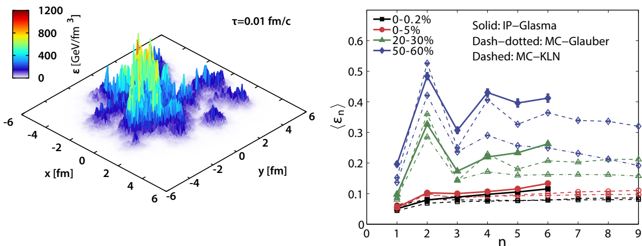
Figure 32. Left: Typical transverse energy density profile for a non-central collision. Right: Primordial fluctuation power spectrum of the matter created in Pb+Pb collisions at the LHC for different centralities, from three different initial state models.
