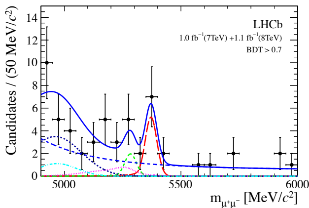
Figure 27. The observed B_s \rightarrow \mu^+ \mu^- signal as seen in the signal region of an optimised boosted decision tree method.
