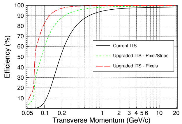
Figure 35. Simulation studies of the tracking efficiency at low transverse momentum with the ITS upgrade (using different types of silicon technologies), compared to the current ITS (black curve). From current studies an improvement of the D^{*+} reconstruction efficiency at low p_T by a factor of about 25 is expected.
