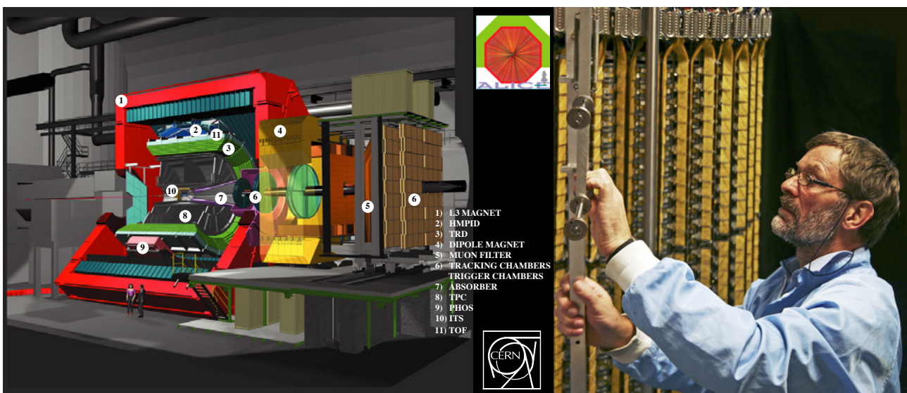
Figure 31. Left: The ALICE detector layout. Right: A Nikhef technician assembling the silicon strip detectors.
