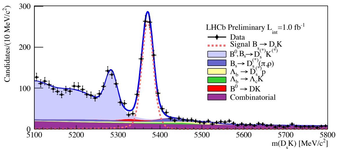
Figure 24. The observed peak of decays of the type B_s \rightarrow D_s K . The signal is shown by the red dotted line, various back-grounds are indicated by the coloured surfaces.
