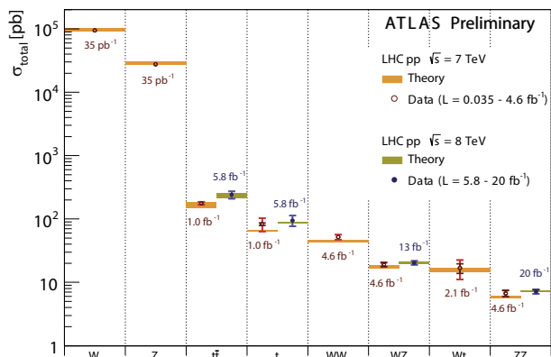
Figure 11. Summary of cross section measurements of important Standard Model processes in the new energy domain of the LHC in Run 1.
