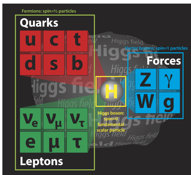
Figure 1. The particles of the Standard Model, including the Higgs boson.
