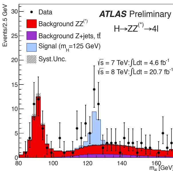
Figure 12. Invariant mass of 4 leptons (left) or 2 photons (right) in the Run 1 ATLAS data, exhibiting a peak that indicates the mass of the Higgs boson around 126 GeV.
