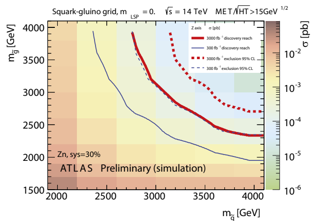
Figure 16. Expected sensitivity, from simulations, for supersymmetric quarks (squarks) and gluons (gluinos), for 300 fb -1 (blue) and 3000 fb -1 (red) at 14 TeV.
