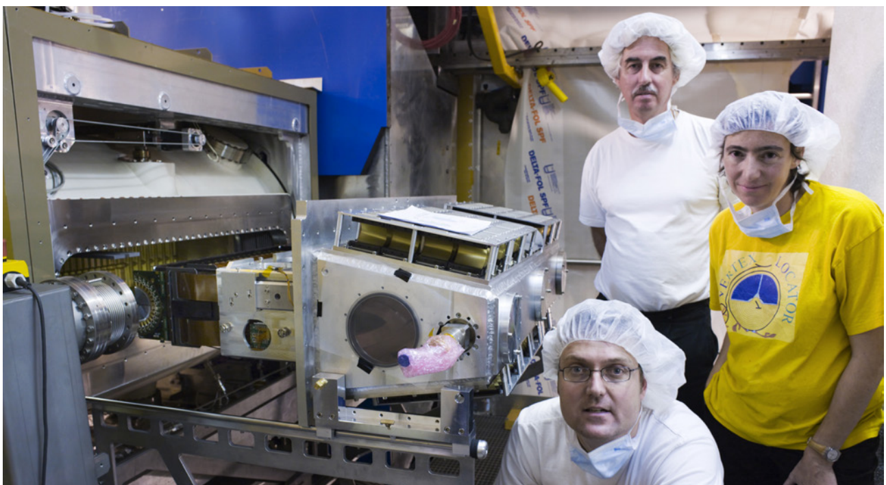
Figure 28. Nikhef technicians install the first half of the LHCb Vertex Locator (VELO) detector.
