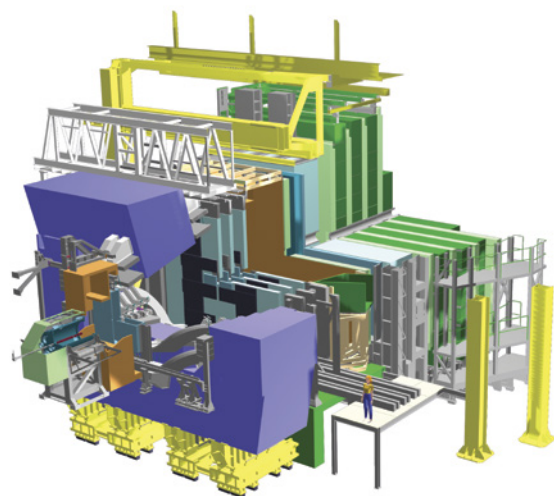
Figure 21. A schematic view of the LHCb detector.
