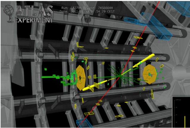
Figure 10. A display of a Higgs boson candidate event recorded by ATLAS. The Higgs boson decays into two Z bosons, which decay in a pair of muons (red) and electrons (yellow).
