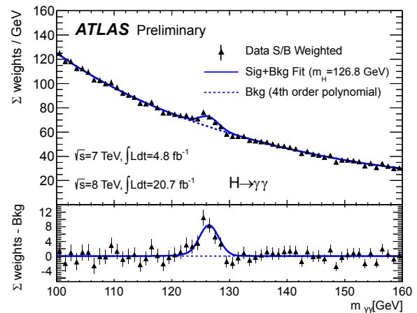
Figure 12. Invariant mass of 4 leptons (left) or 2 photons (right) in the Run 1 ATLAS data, exhibiting a peak that indicates the mass of the Higgs boson around 126 GeV.
