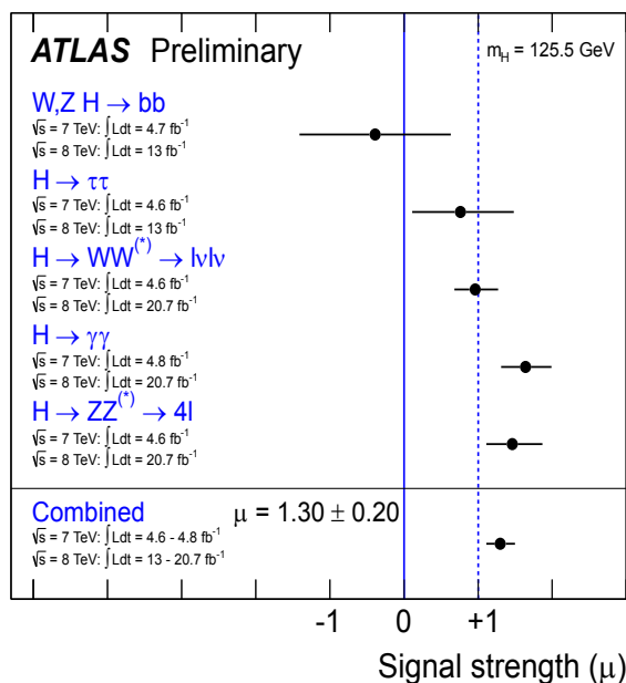
Figure 13. Measured Higgs boson signal strength, normalised to the Standard Model prediction, in Run 1 ATLAS data in various Higgs decay channels.
