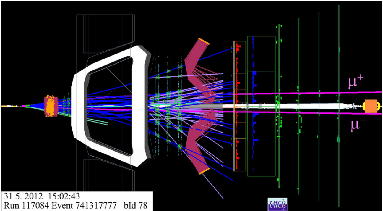
Figure 26. Graphic representation of a B_s \rightarrow \mu^+ \mu^- event candidate. This figure shows the detector hits and the reconstructed particle trajectories as blue curves. The two muon tracks are shown in purple.
