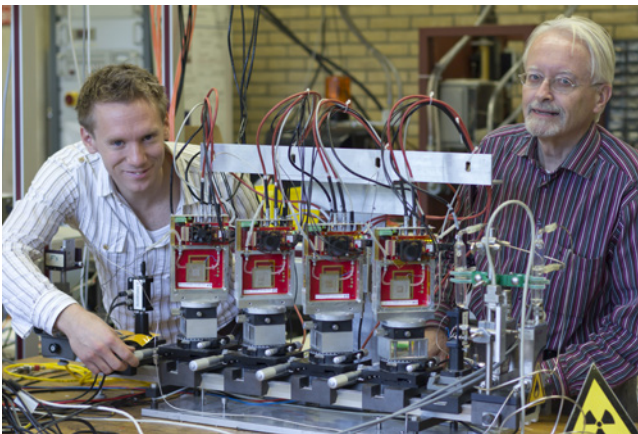
Figure 18. Development of new technology at Nikhef for a future ATLAS inner tracker.
