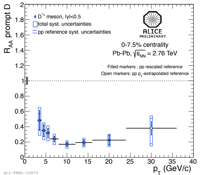
Figure 34. Nuclear modification factor R_{AA} of the D^{*+} meson as function of transverse momentum.
