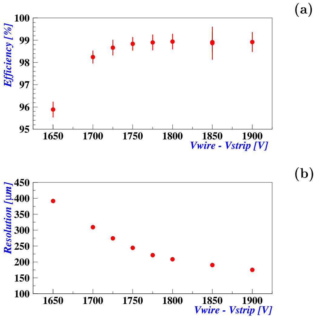
Fig. 9. Behaviour of the single wire efficiency (estimated as described in the text) (a) and resolution (b) as a function of V_{ampl} = V_{wire} - V_{strip} . The I beams were set at -1.2 kV.
