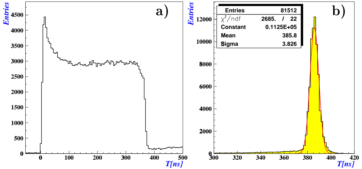
Fig. 8. A TDC spectrum as obtained from the raw data in a typical run during the test beam period can be seen in (a). A meantimer (MT) distribution can be seen in (b) together with the result of a gaussian fit providing a sigma of 3.8 ns. From this value an average spatial resolution of 170 \mu\text{m} can be computed. The position of the MT peak allows to obtain an average drift velocity of 54.4 \mu\text{m}/\text{ns} . The tail on the left of the peak is due to delta rays.
