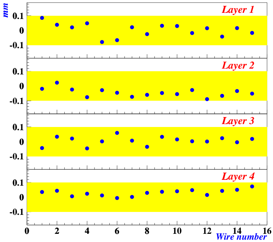
Fig. 7. Deviations from the nominal pitch of wires in each of the Q4 layers from measurements using a CCD camera as explained in the text. In all cases, the wires are inside the \pm 100 \mu\text{m} window as required.
