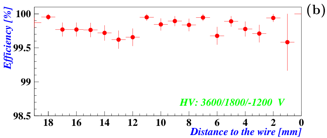
Fig. 13. Efficiency as a function of the distance to the wire (a); with an expanded scale excluding the I-beam region (b).
