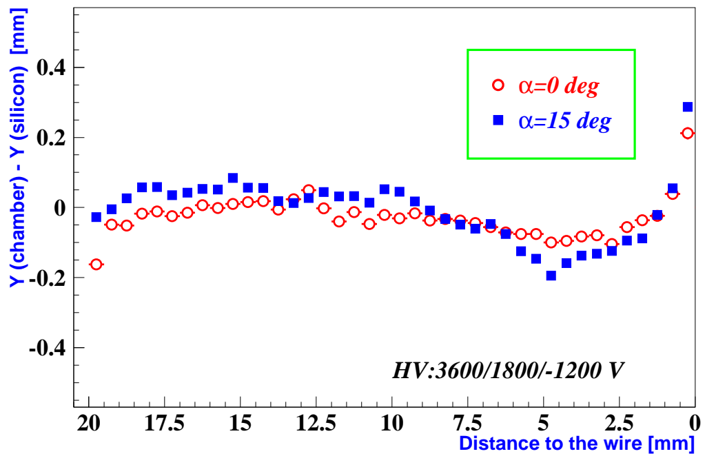
Fig. 11. Deviations from linearity as a function of the distance to the wire for tracks with \alpha = 0 and \alpha = 15 degrees. The I-beam is centered at 21 mm.
