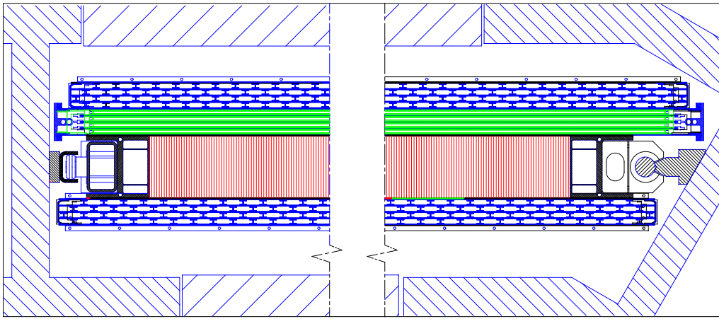
Fig. 1. Cut view of a drift tube chamber in its final position inside the CMS iron yoke. Two superlayers with wires along the beam direction and a third crossed one can be seen as well as the honeycomb panel providing rigidity to the chamber.
