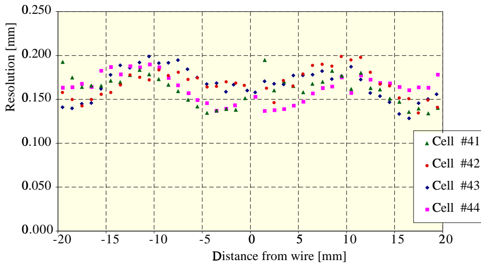
Fig. 12. Resolution as a function of the distance to the wire for a few different cells. The values obtained are in the range 0.15 to 0.2 mm and are rather uniform in all cells.
