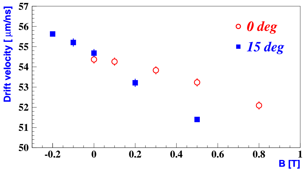
Fig. 17. Drift velocity for several magnetic fields for perpendicular (0 deg) and inclined (15 deg) tracks.
