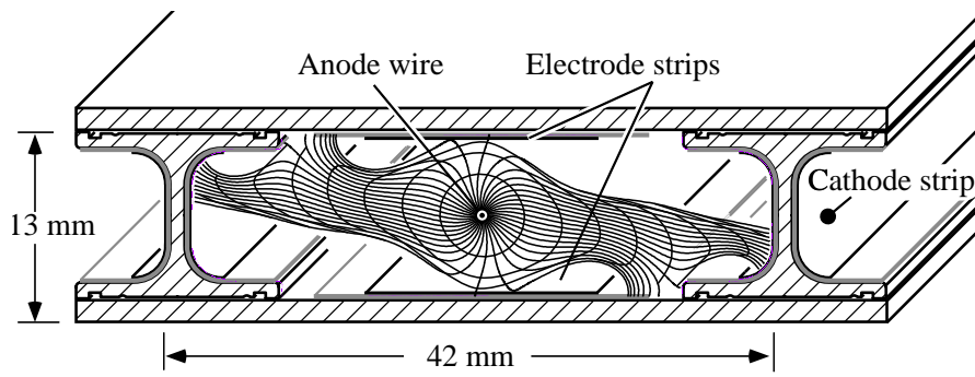
Fig. 16. Simulation of the distortion produced in the drift lines by a 0.5 T magnetic field parallel to the wires.
