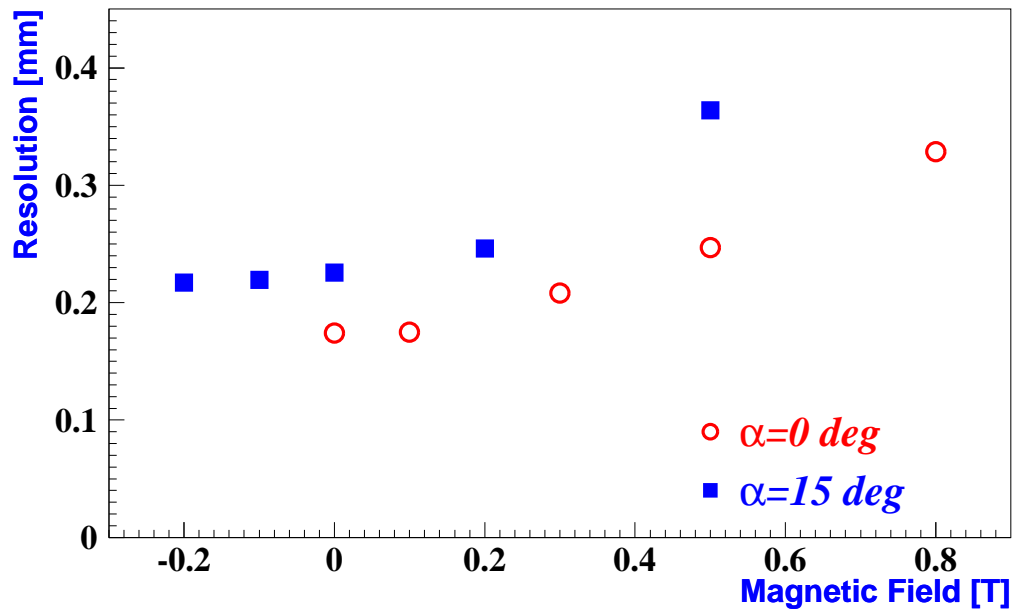
Fig. 19. Single cell resolution as a function of the magnetic field parallel to the wires for tracks with \alpha = 0 and \alpha = 15 degrees. The constant average drift velocity of Fig. 17 is used for time to space conversion for each field value.
